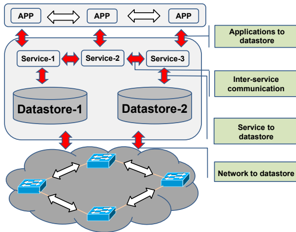
Figure 2: Threat model.
