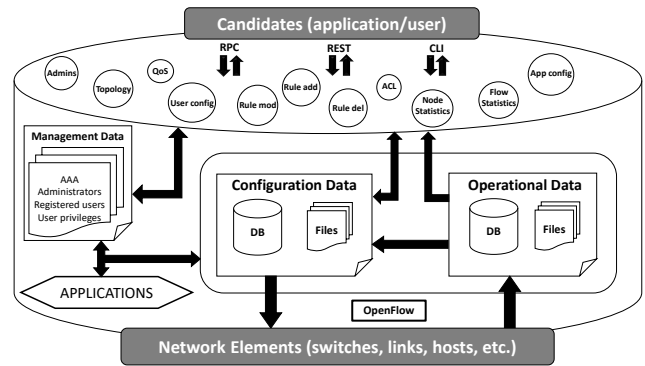
Figure 1: The constitution of SDN: Applications store network configuration in controller, controller configures the network and provides operational state back to applications
