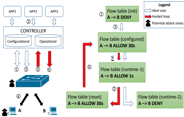
Figure 6: Configuration poisoning attack: an attacker compromises the flow table and establishes a hacked loop to indefinitely allow communication in the network.
